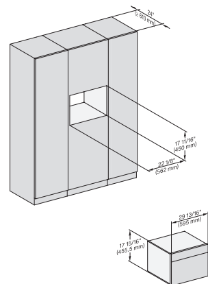
DGC7x4x, H7x40BM, Einabu, 30 Zoll, Proud, 450S
