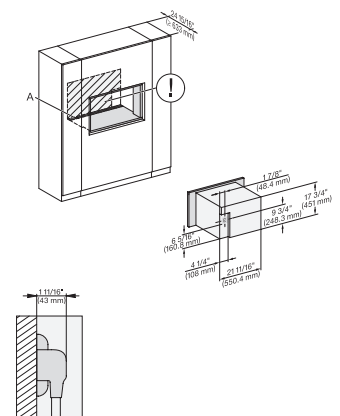
DGC7x4x(+EBA7848), Installation, 30 Zoll, Flush inset, wide front, XL
