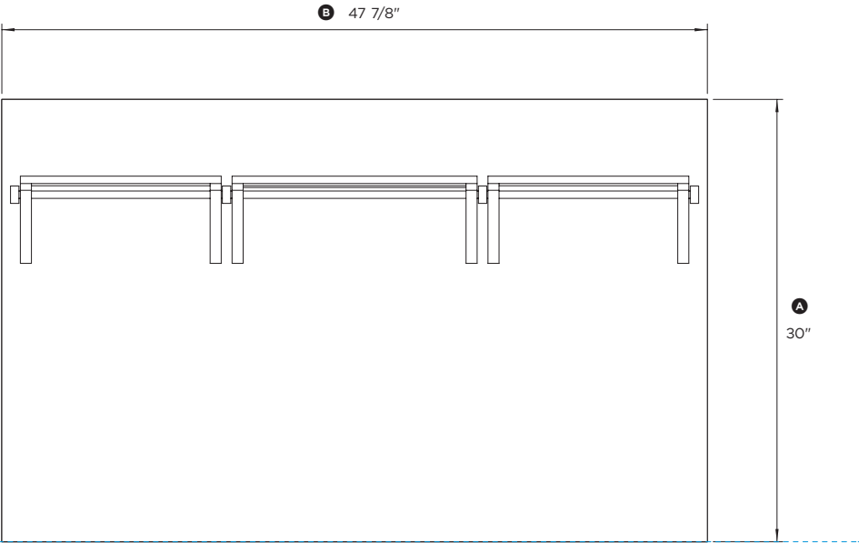
PLAN VIEW
