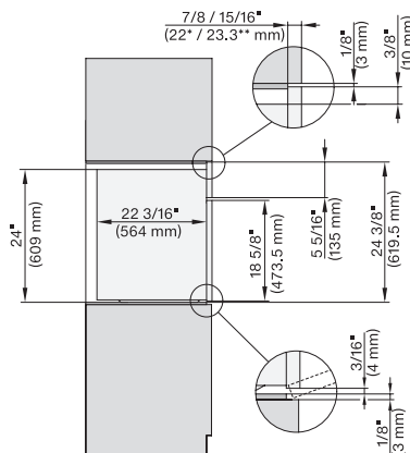
DGC7x8(X), side view, 30 Zoll, Flush inset, XXL
