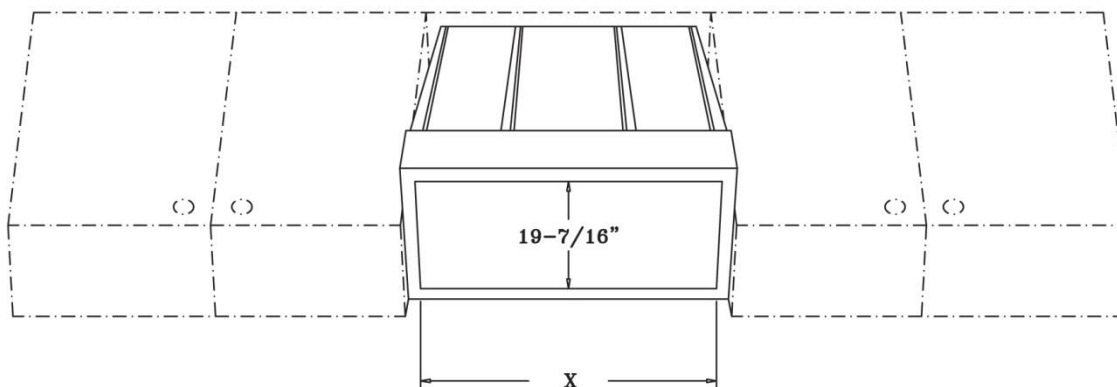
SIZE OF THE CUT OUT - (BOTTOM VIEW)
