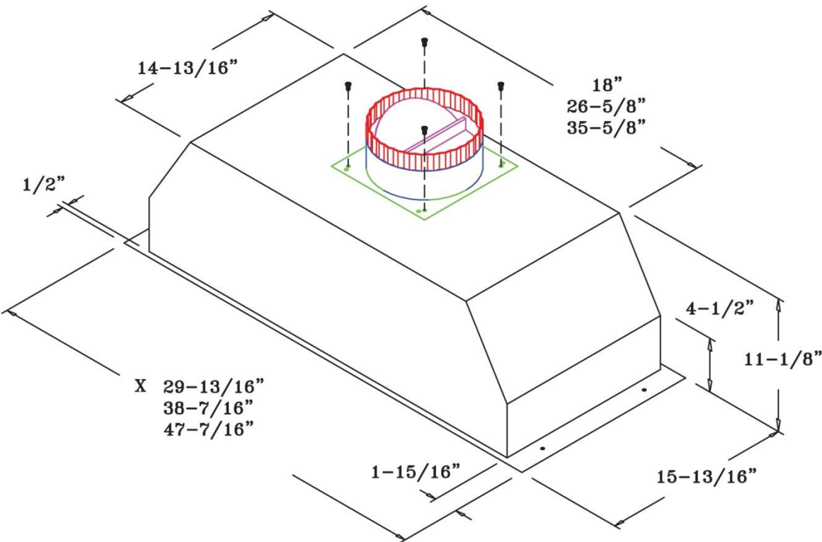
POSITION OF 8" ROUND COLLAR (TOP VIEW)
