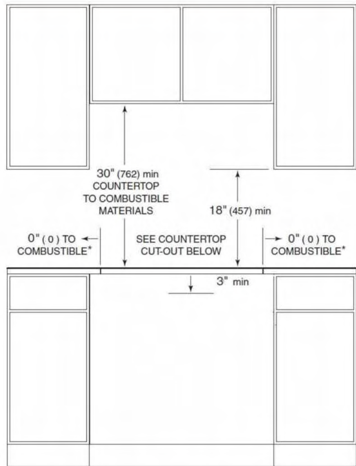
FRONT VIEW
