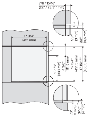
CVA7440, CVA7840, installation drawing, side view, 60 cm, Flush inset, NA
