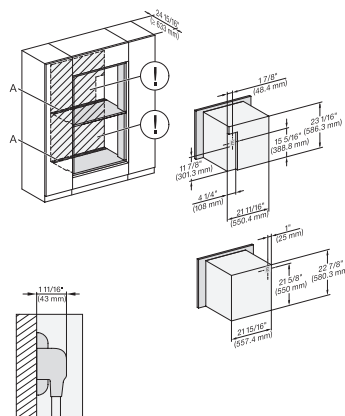
DGC786x+EBA7868, H7x6xBP(+EBA7848), Instllation, 30 Zoll, Flush inset, combi, XXL, 650S
