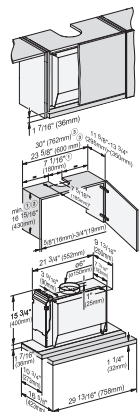
DAS4720 US, Installation drawings, VG USA
