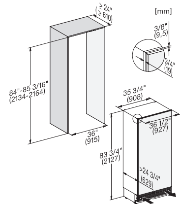
K2902SF, K2912SF, F2912SF, K2901SF, K2911SF, F2911SF, K2901 SF, K2911 SF, F2911 SF, inner space, MasterCool (US, CA)
