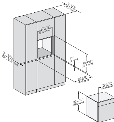
DGC786x H7x6xBP, Einbau, 30 Zoll, Flush inset, 650S 7/8" – 22" mm – Glass, 15/16" – 23.3" mm – Stainless steel
