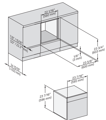
H7x6xBP, Einbau, 30 Zoll, Flush inset, built-under 7/8" – 22" mm – Glass, 15/16" – 23.3" mm – Stainless steel
