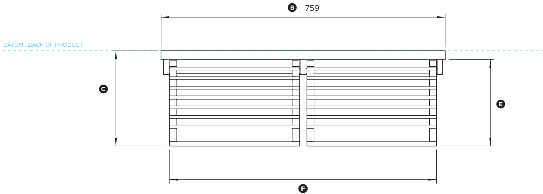
PLAN VIEW
