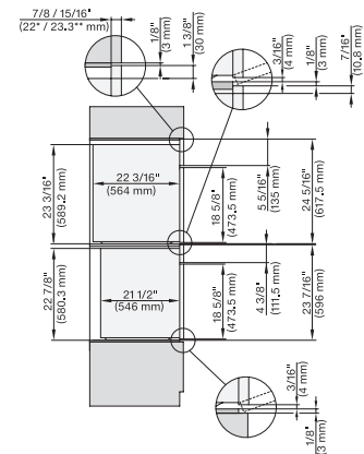
DGC7x8x(X), H7x6x(+EBA7868), side view, 30 Zoll, Flush inset, combi, XXL, 650S
