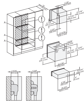
DGC786x+EBA7868, H7x80BP, ESW7x80, Installation, 30 Zoll, Proud, combi, XXL, 650
