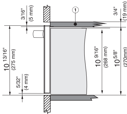
ESW 6*80, CLST (detailed installation drawing) – USA
