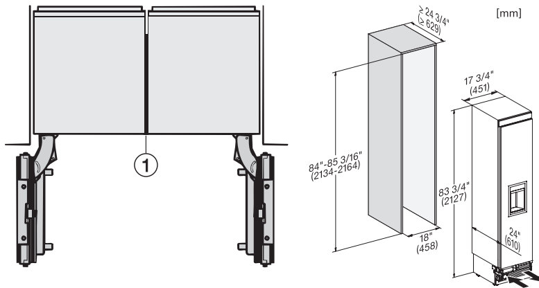
Side-by-side, MasterCool, without partition wall, with heating mat (Sketch) (with footnote)
