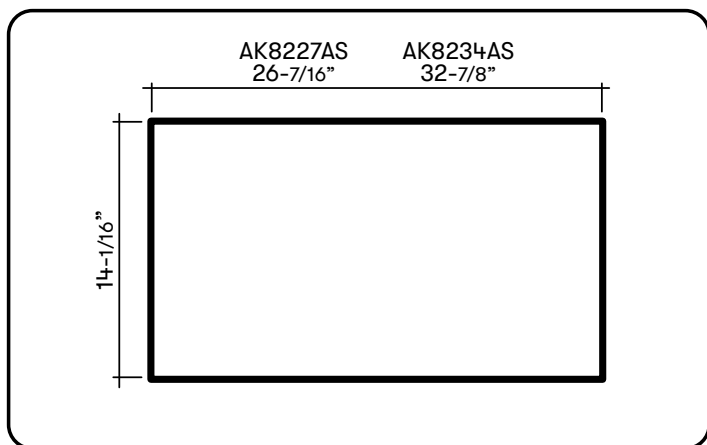
Cabinet Bottom Cut-Out Size (W x D): 26-7/16" x 14-1/16" (AK8227AS), 32-7/8" x 14-1/16" (AK8234AS)
