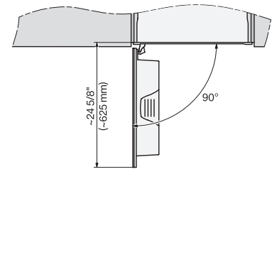
CVA7440, CVA7445, CVA7840, CVA7845, installation drawing, view from above, 60 cm, Flush inset
