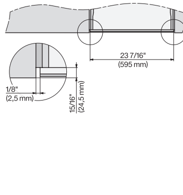
CVA7440, CVA7445, CVA7840, CVA7845, installation drawing, view from above, 60 cm, Flush inset
