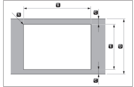
Fig. 11.10 Cut-out dimensions for surface mounting
