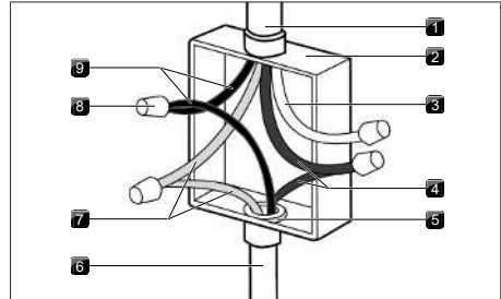
Fig. 11.20 4-Wire Cable
