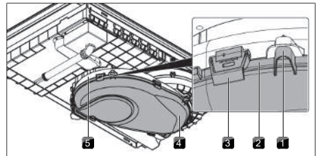
Fig. 9.2 Air guiding housing
