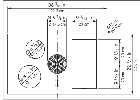
Fig. 5.4 Appliance dimensions top view
