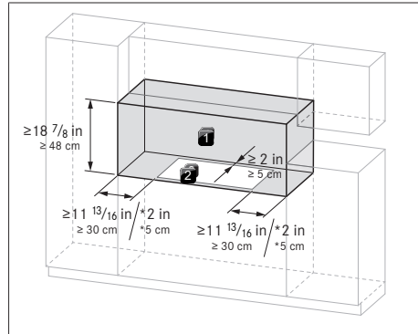
Fig. 11.3 Distance requise
