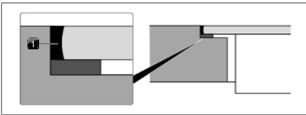
Fig. 11.27 Silicone sealant for flush installation
