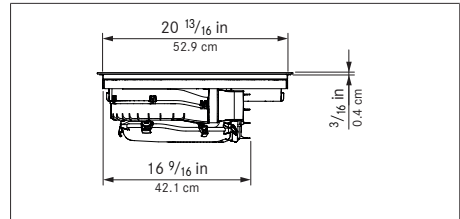
Fig. 5.6 Appliance dimensions side view
