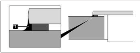
Fig. 11.26 Silicone sealant for surface mounting
