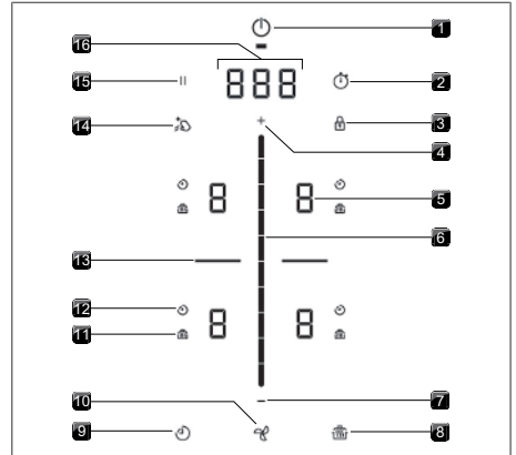
Fig. 6.3 Operating panel
