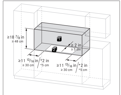
Fig. 11.3 Required clearance
