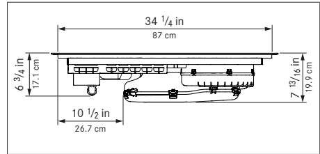
Fig. 5.5 Appliance dimensions front view
