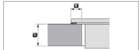
Fig. 11.11 Overlay dimensions for surface mounting
