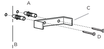
C. Vent cover support bracket D. 5 x 45 mm screws
