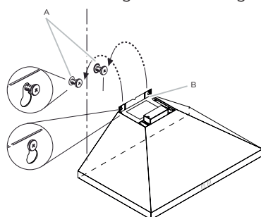
A. Mounting screws B. Mounting slots
