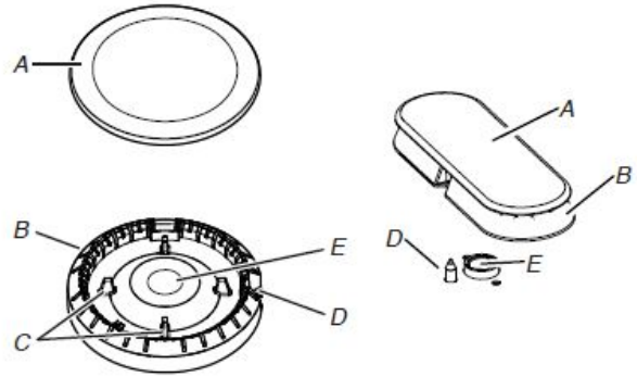
A. Burner cap D. Igniter B. Burner base E. Gas tube opening C. Alignment pins
