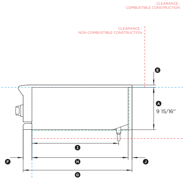
PROFILE VIEW
